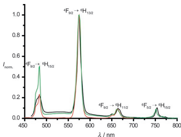
Figure 3. Emission spectra with transition assignment of 1 (green), 2 (red), and 3 (black) at room temperature under excitation at \lambda_{\text{ex}} = 453 nm.
