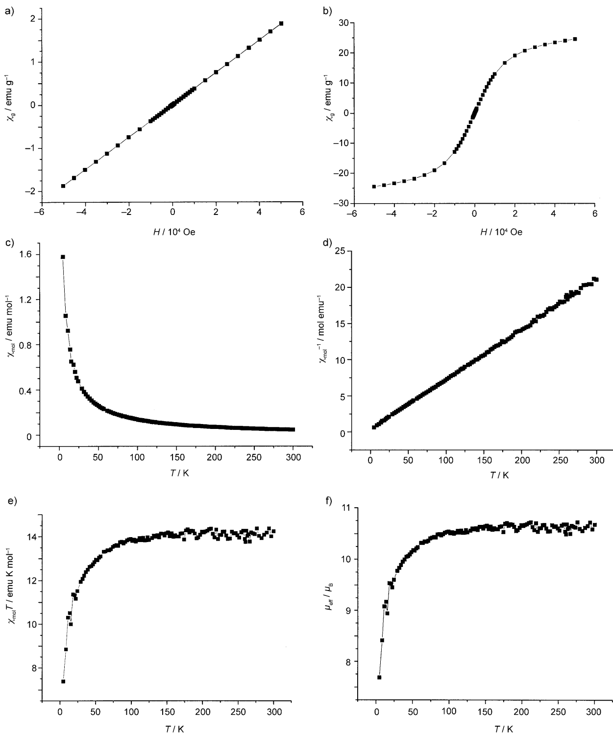
Figure 2. Field dependence of the mass susceptibility \chi_{\text{g}} at a) 300 K and b) 5 K. Temperature dependence of c) the static molar susceptibility and d) the reciprocal molar susceptibility at a field of 10000 Oe. Temperature dependence of e) the product of the temperature and the static molar susceptibility and f) the effective magnetic moment at a field of 10000 Oe for 2 .
